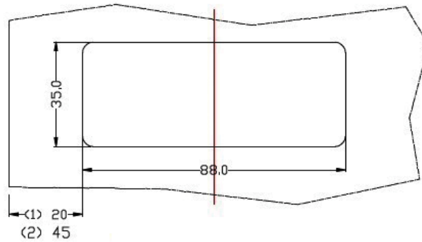
HOLE DIMENSION Measurement: mm
