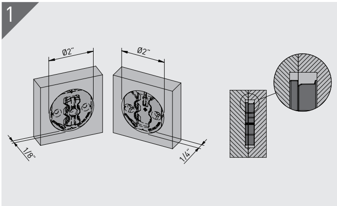
Part Rebate - each substrate mounting face is rebating as shown. Ensure sufficient screw embedment in substrate.
