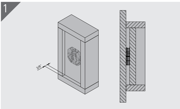
Setting back the mounting face of either the Hook (as shown) or Key by 9.5mm results in a concealed joint without the need to cut rebates.
