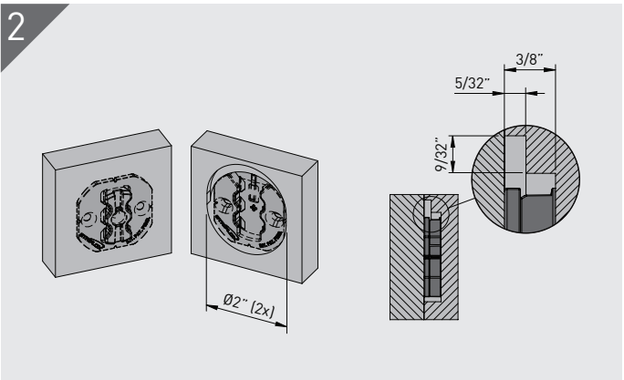
Full Rebate - 1 of the substrate mounting faces is rebating the full depth as shown. Ensure sufficient screw embedment in substrate.
