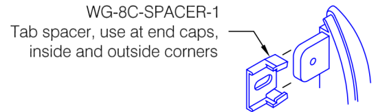
Spacer Detail
